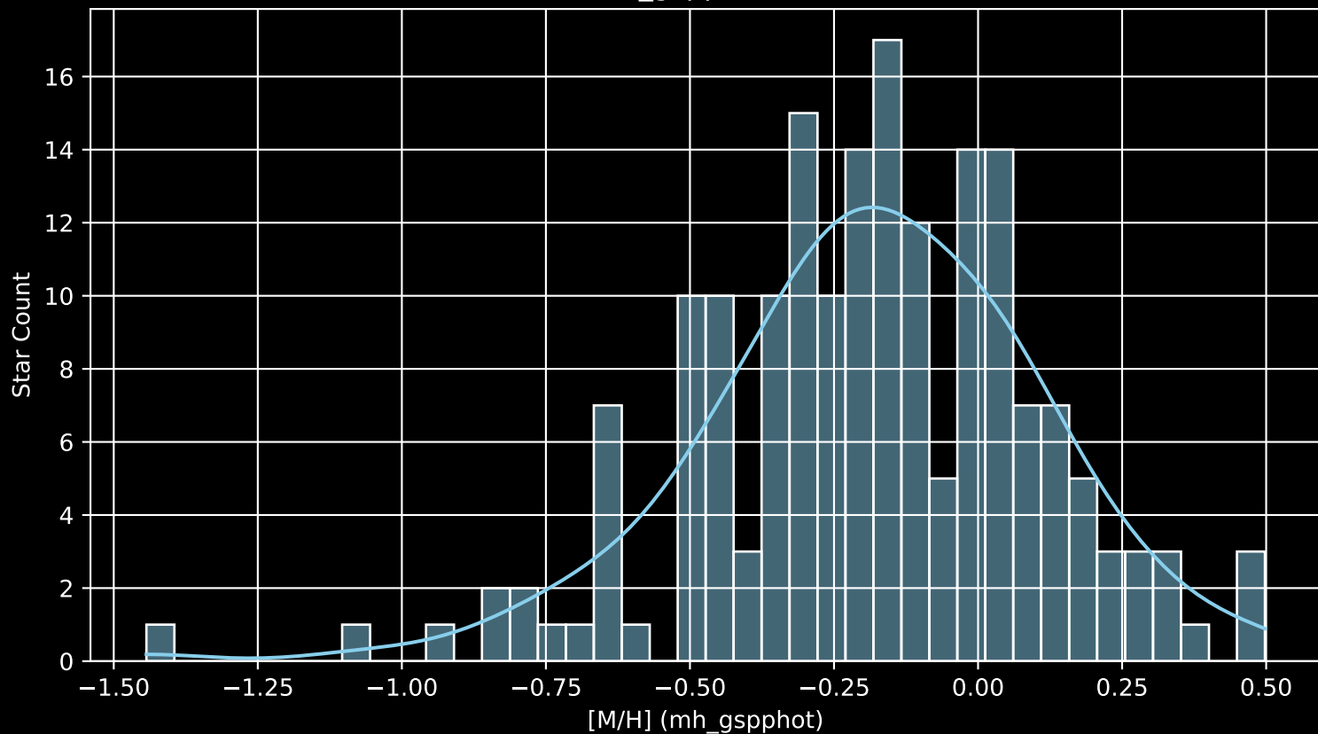
APOGEE DR17 Field: [106+60_MGA [M/H] (mh_gspphot) (n= 183)
