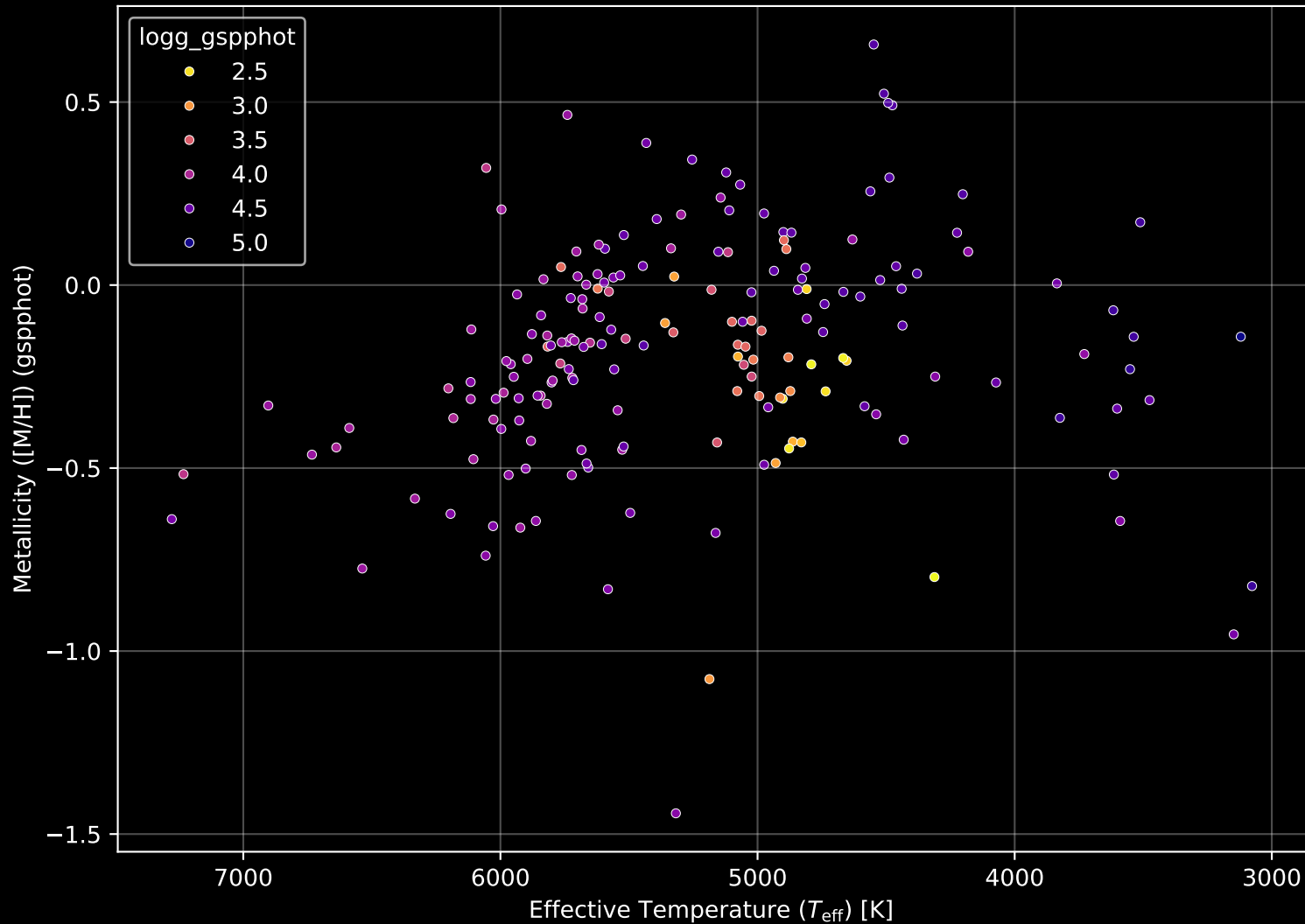
APOGEE DR17 Field: [106+60_MGA] Stellar Population Parameters (n= 185)
