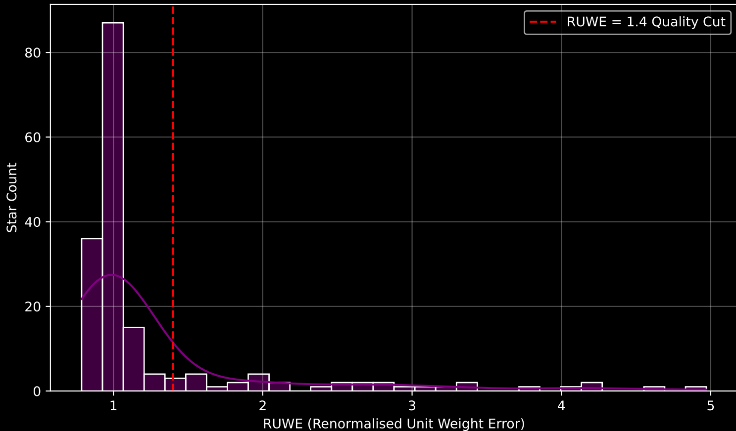
GAPOGEE DR17 Field [106+60_MGA] RUWE Distribution (n= 176)
