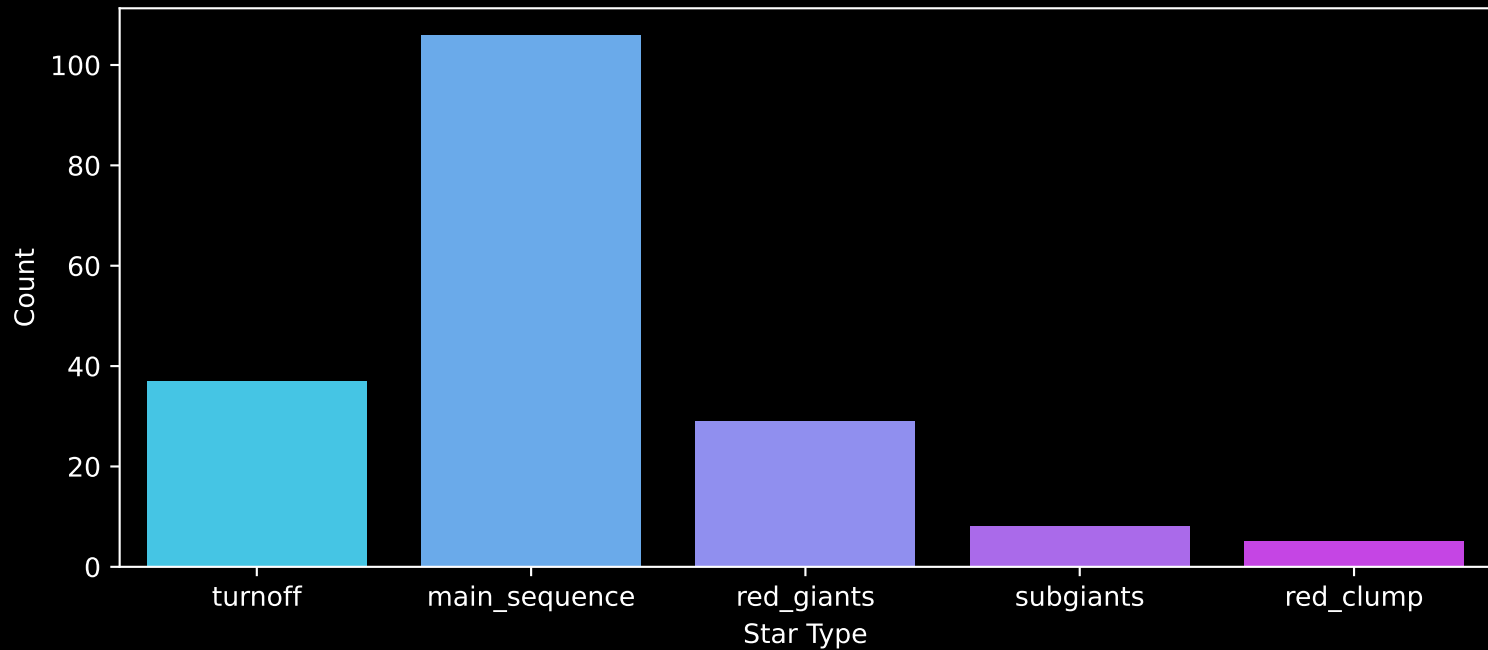
APOGEE DR17 Field: [106+60_MGA] Count plot of Star Type
