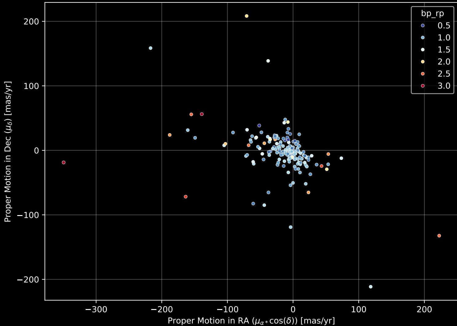
APOGEE DR17 Field: [106+60_MGA] Proper Motion Diagram (n= 185)
