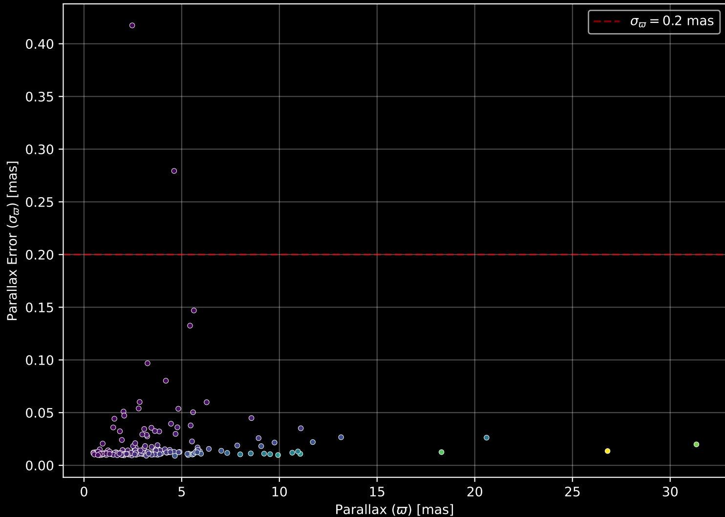
APOGEE DR17 Field: [106+60_MGA] Parallax Quality (n= 185)
